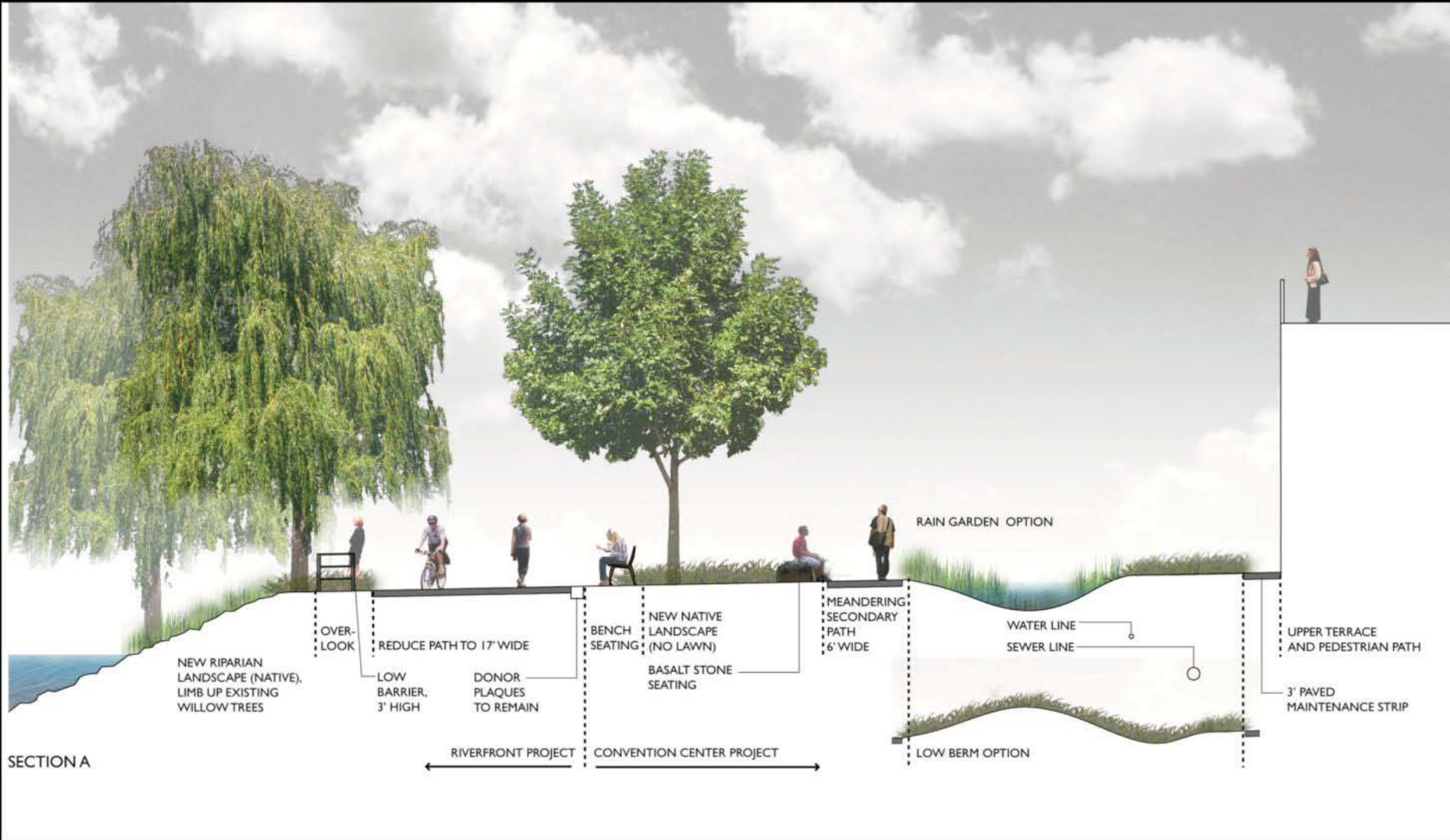
SECTION "A" -- AT ADDITION
